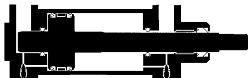
Non-magnetic piston
