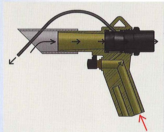
Illustration showing air flow, blowing and vacuuming simultaneously.
